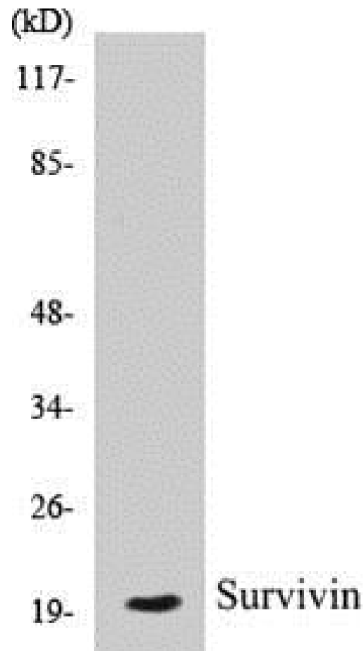
Figure 4. Western blot analysis of extracts from mouse lung cells, using the Anti-Survivin Antibody.
