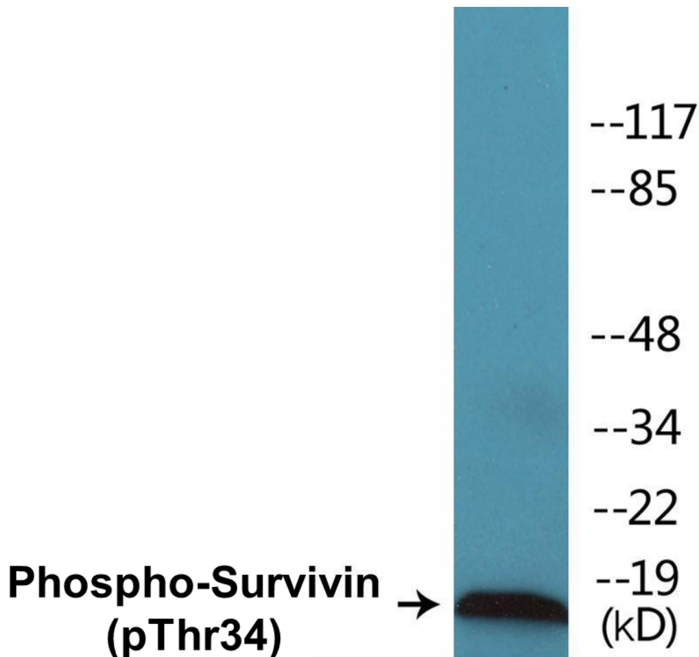
Figure 2. Western blot analysis of extracts from HT29 cells treated with EGF 100ug/ml 30', using the Anti-Survivin (Phospho-Thr34) Antibody
