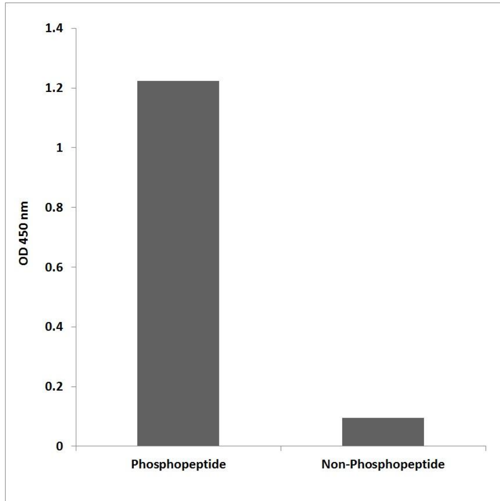
Figure 3. Enzyme-Linked Immunosorbent Assay (ELISA) for immunogen phosphor-peptide (left) and non-phospho peptide (right), using Anti-Survivin (Phospho-Thr34) Antibody.
