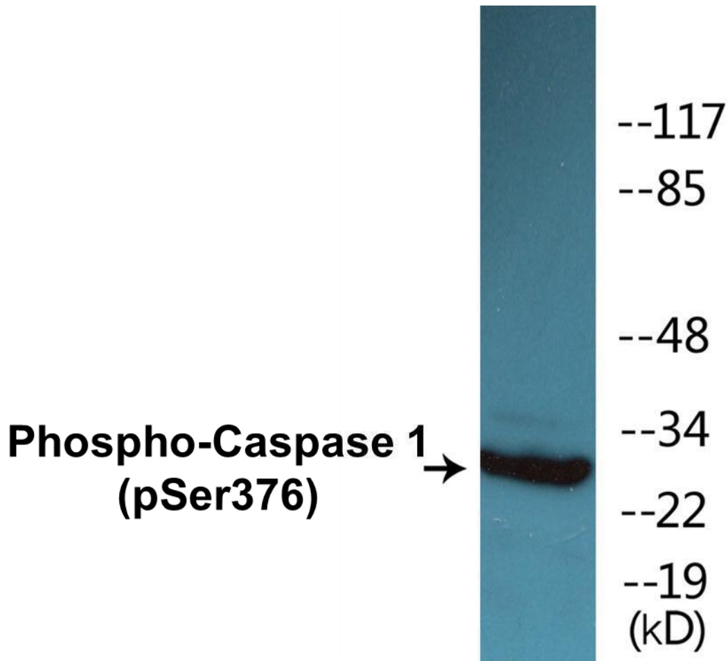
Figure 2. Western blot analysis of extracts from 293 cells, using the Anti-Caspase 1 (Phospho-Ser376) Antibody.
