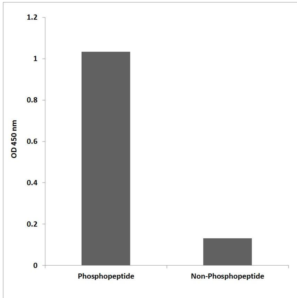
Figure 3. Enzyme-Linked Immunosorbent Assay (ELISA) for immunogen phosphor-peptide (left) and non-phospho peptide (right), using Anti-Caspase 1 (Phospho-Ser376) Antibody.
