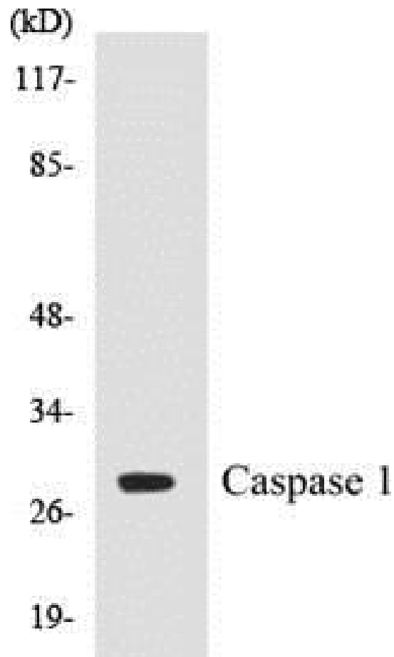
Figure 4. Western blot analysis of extracts from 293/MCF-7/HeLa cells, using the Anti-Caspase 1 Antibody.
