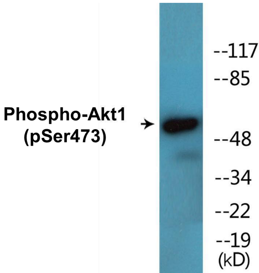
Figure 2. Western blot analysis of extracts from HeLa cells treated with heat shock, using the Anti-Akt1 (Phospho-Ser473) Antibody.
