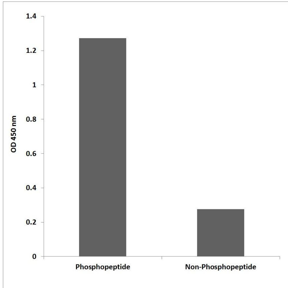
Figure 3. Enzyme-Linked Immunosorbent Assay (ELISA) for immunogen phosphor-peptide (left) and non-phospho peptide (right), using Anti-Akt1 (Phospho-Ser473) Antibody.
