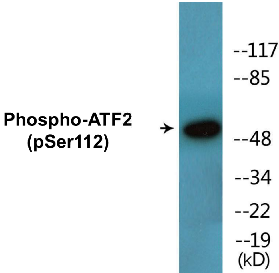
Figure 2. Western blot analysis of extracts from MDA-MB-435 cells, using the Anti-ATF2 (Phospho-Ser112) Antibody.
