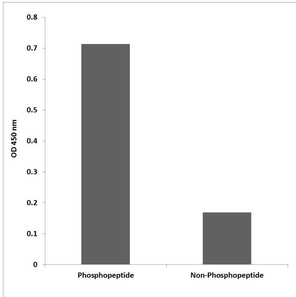
Figure 3. Enzyme-Linked Immunosorbent Assay (ELISA) for immunogen phosphor-peptide (left) and non-phospho peptide (right), using Anti-ATF2 (Phospho-Ser112) Antibody.
