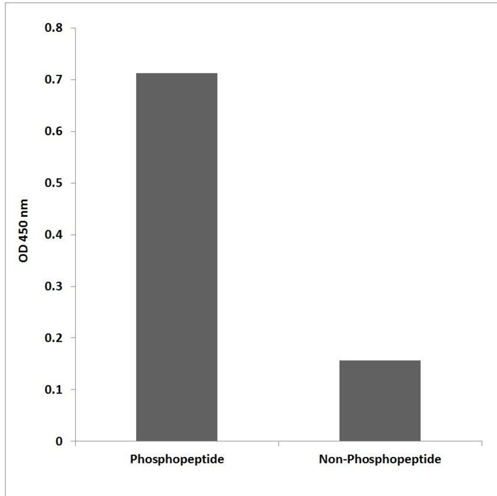
Figure 3. Enzyme-Linked Immunosorbent Assay (ELISA) for immunogen phosphor-peptide (left) and non-phospho peptide (right), using Anti-Integrin \beta 3 (Phospho-Tyr773) Antibody.
