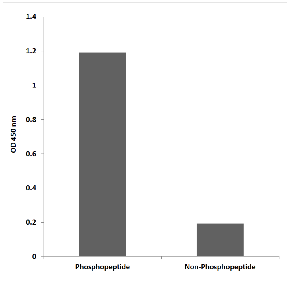
Figure 3. Enzyme-Linked Immunosorbent Assay (ELISA) for immunogen phosphor-peptide (left) and non-phospho peptide (right), using Anti-STAT1 (Phospho-Tyr701) Antibody.
