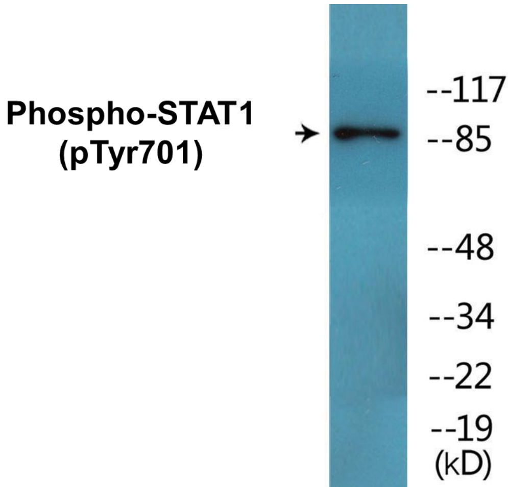
Figure 2. Western blot analysis of extracts from COS7 cells using the Anti-STAT1 (Phospho-Tyr701) Antibody.
