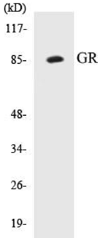
Figure 2. Western blot analysis of extracts from Jurkat cells, treated with PMA 125ng/ml 30', using GR (Ab-203) Antibody.
